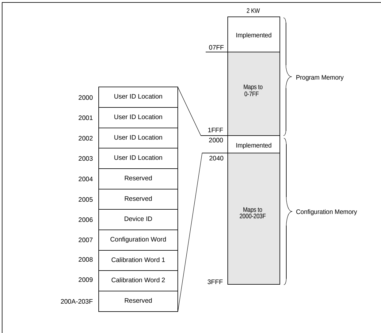
FIGURE 2-3: PIC16F636/639 PROGRAM MEMORY MAPPING
